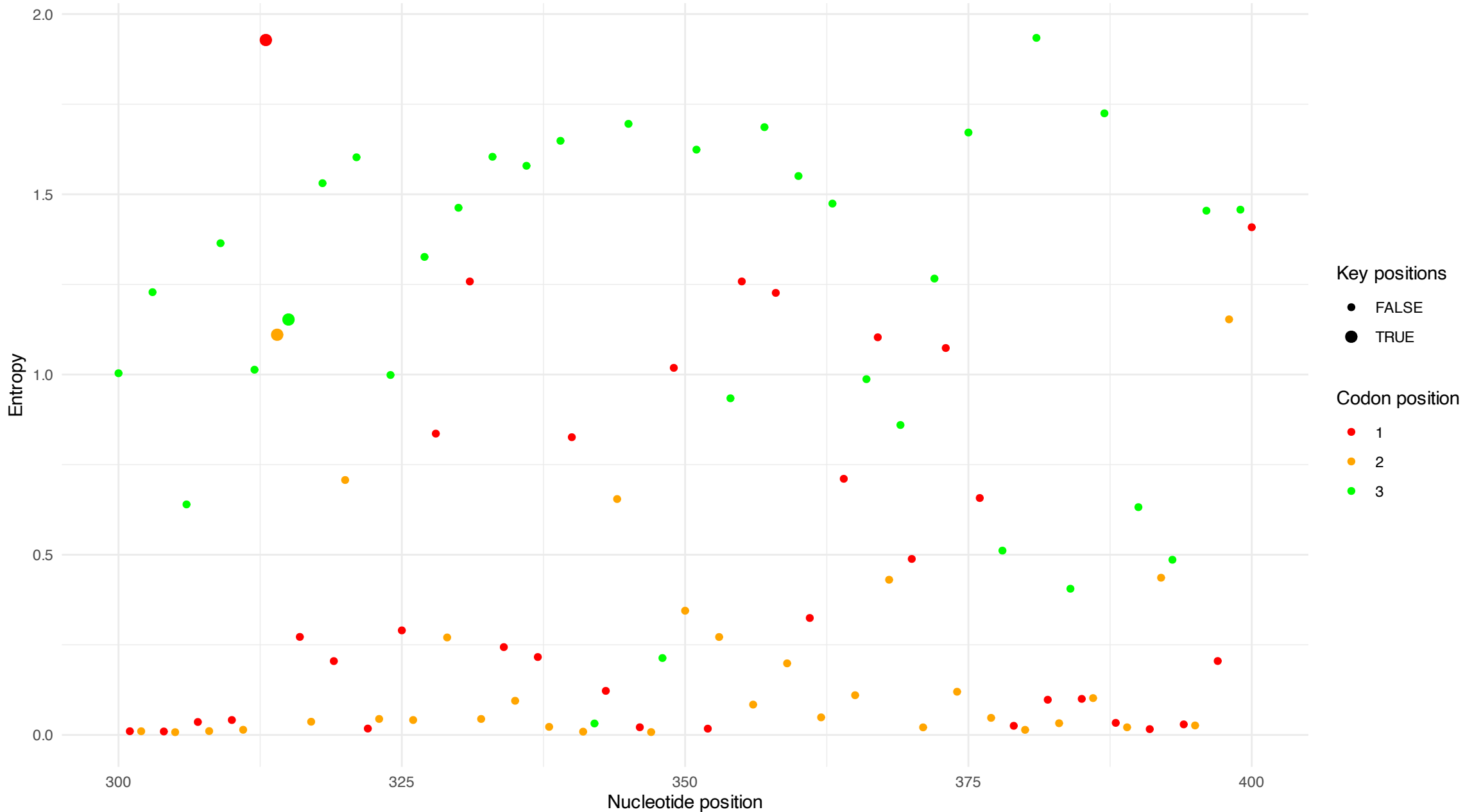
Entropy across positions 300-400 (105_I_ATC_0)
