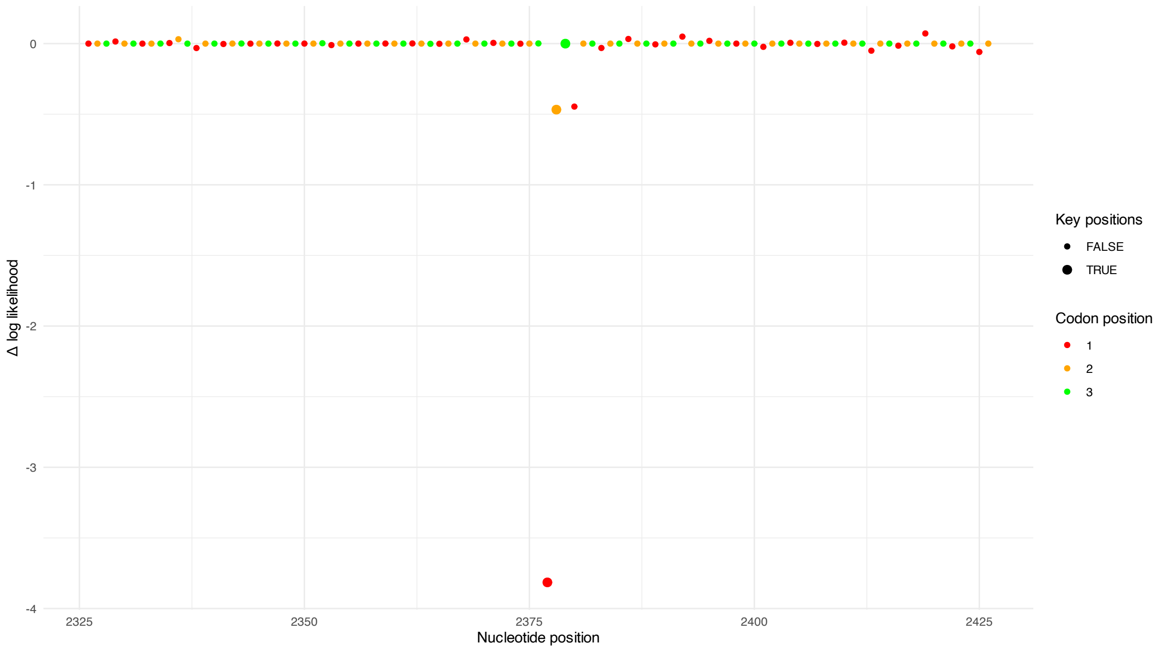
log likelihood difference: 83_AGT_rc vs 83_AGC_rc
