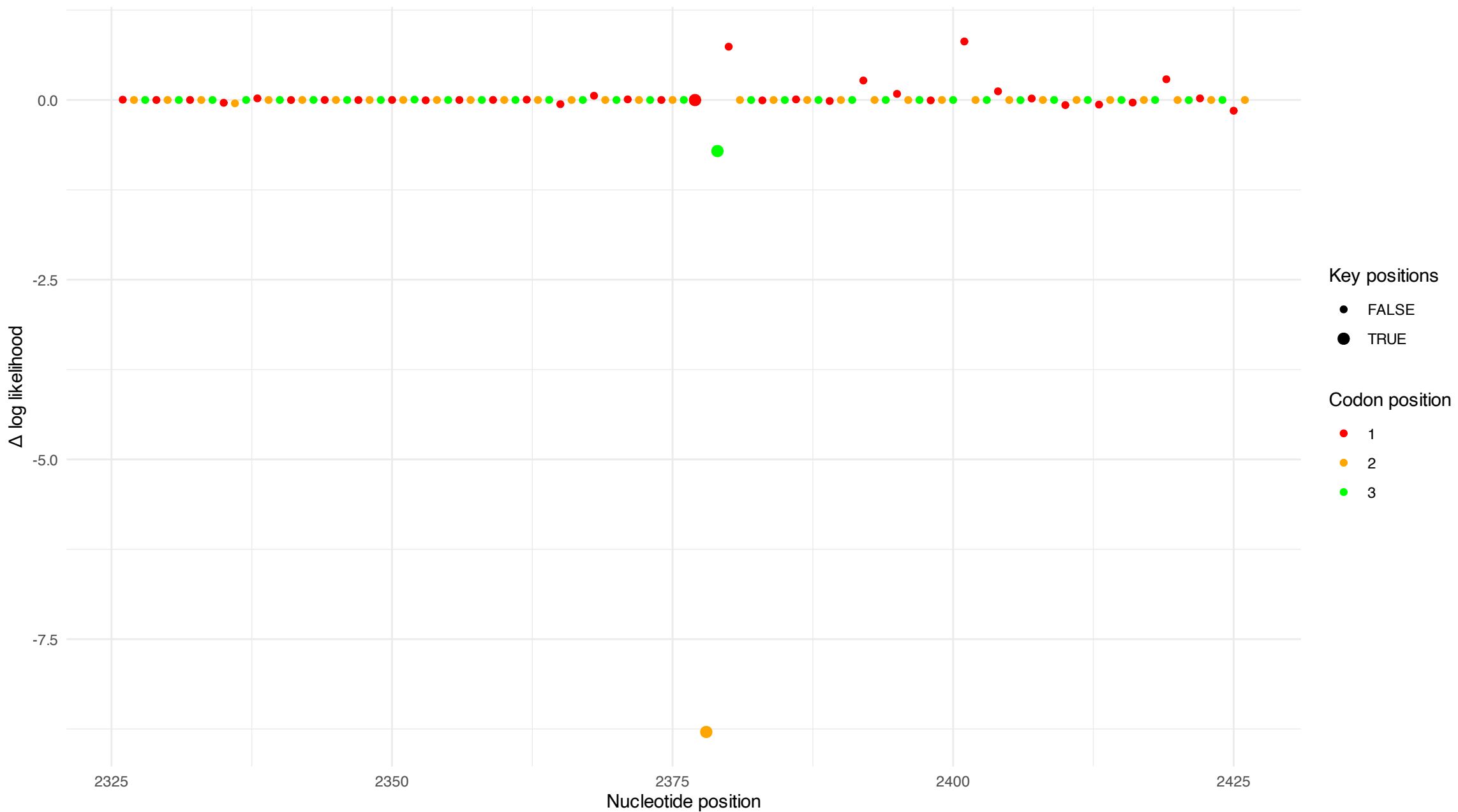
log likelihood difference: 83_ATC_rc vs 83_AGC_rc
