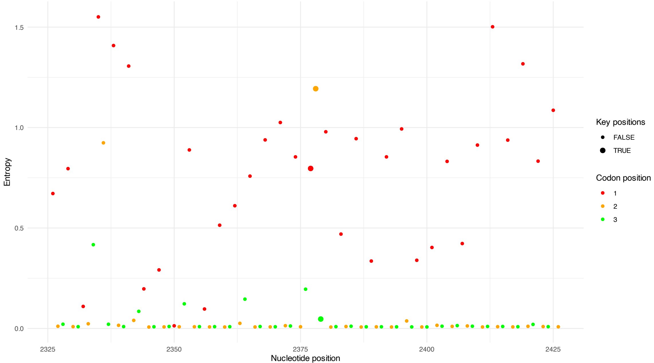
Entropy across positions 2326-2426 (83_AGT_rc)
