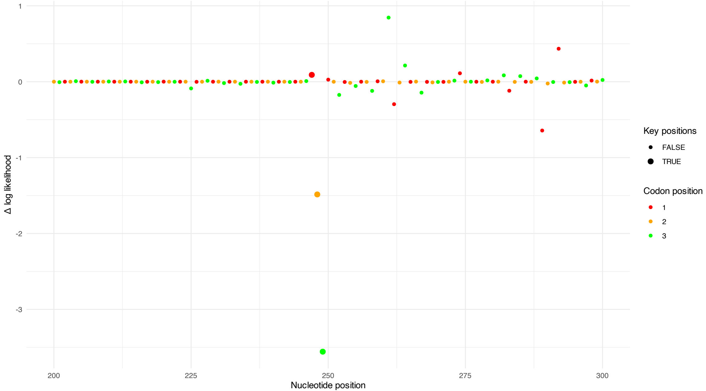
log likelihood difference: 83_L vs 83_S1
