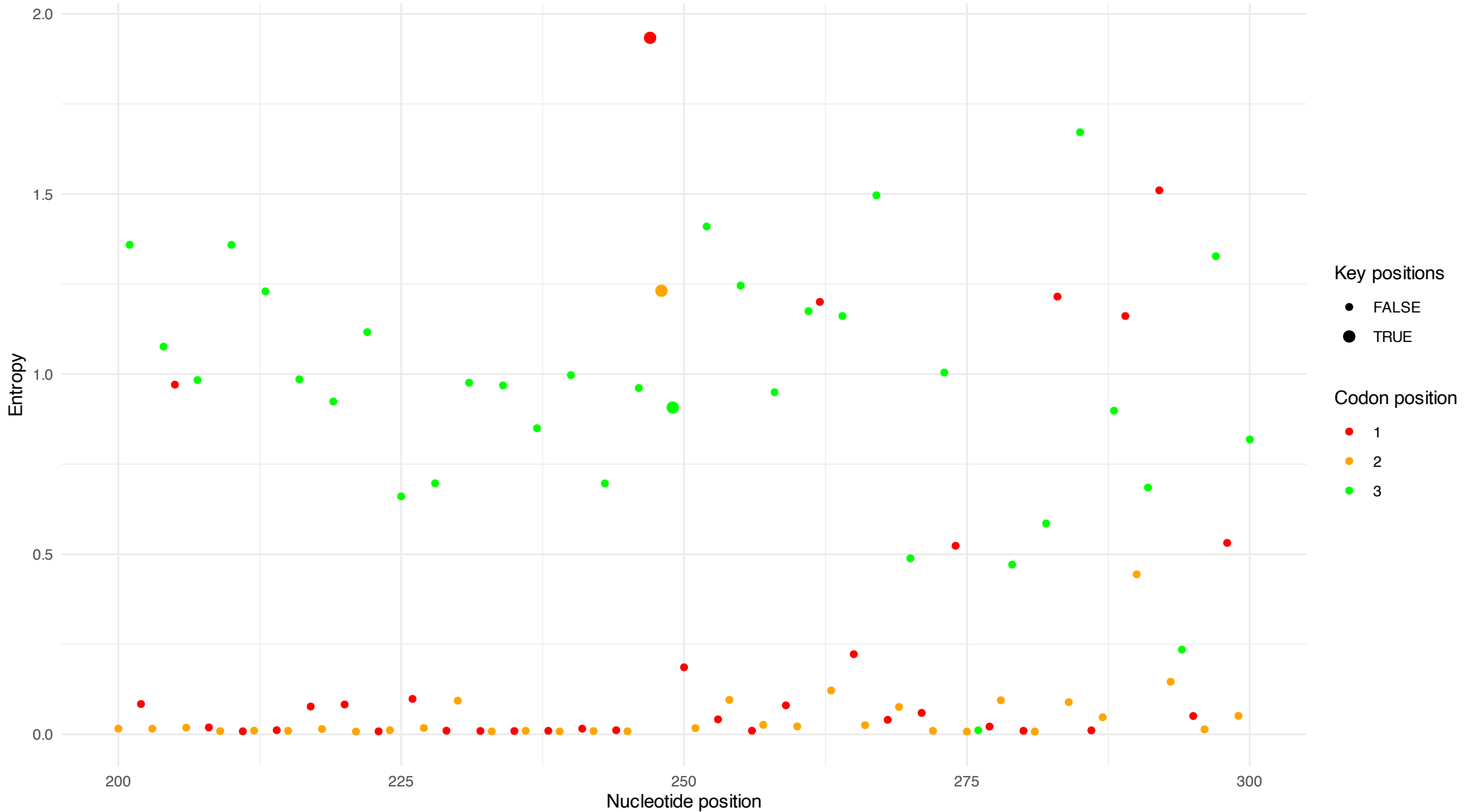
Entropy across positions 200-300 (83_L)
