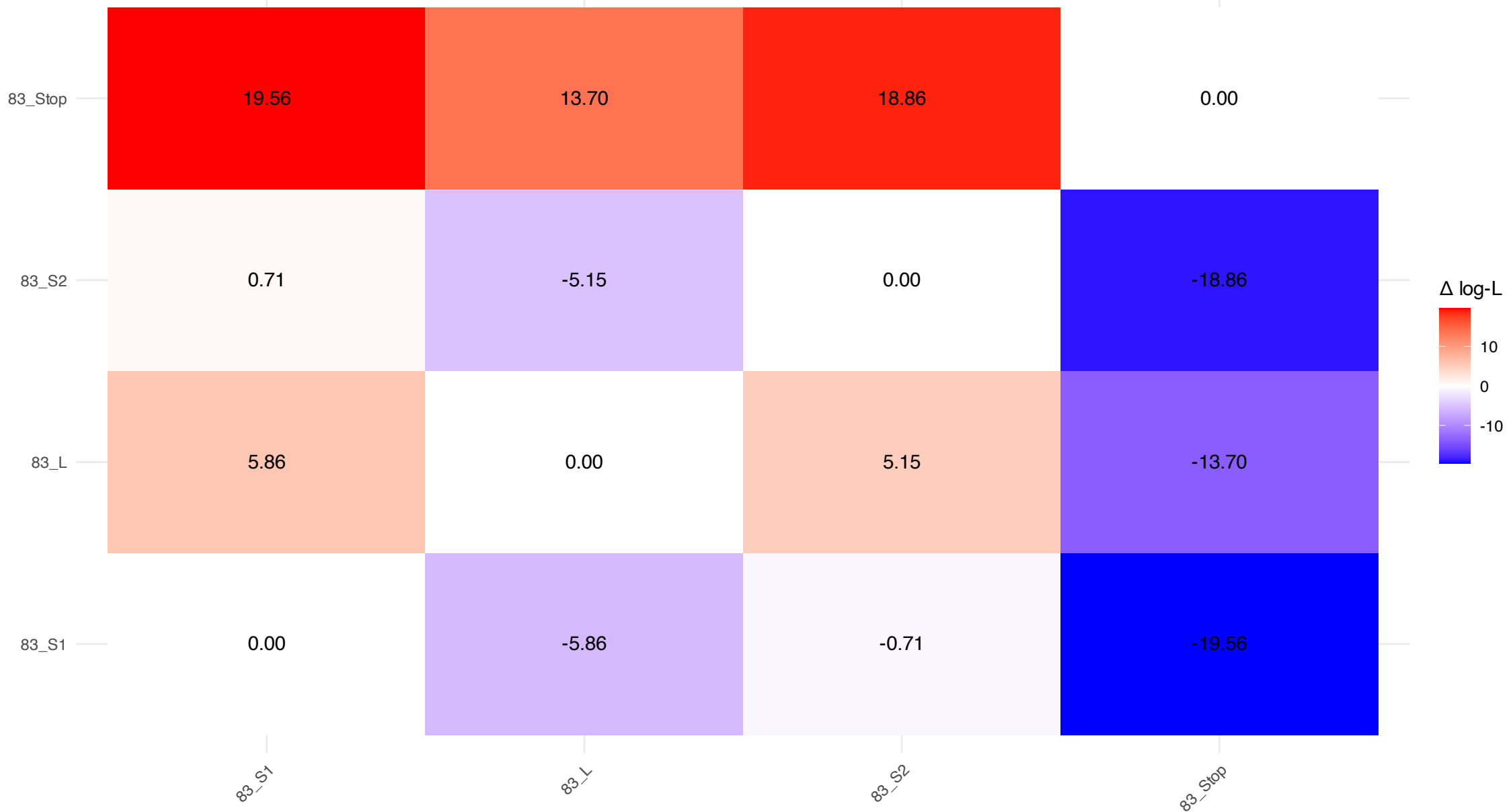
Log-Likelihood Differences Between Variants (col-row)
