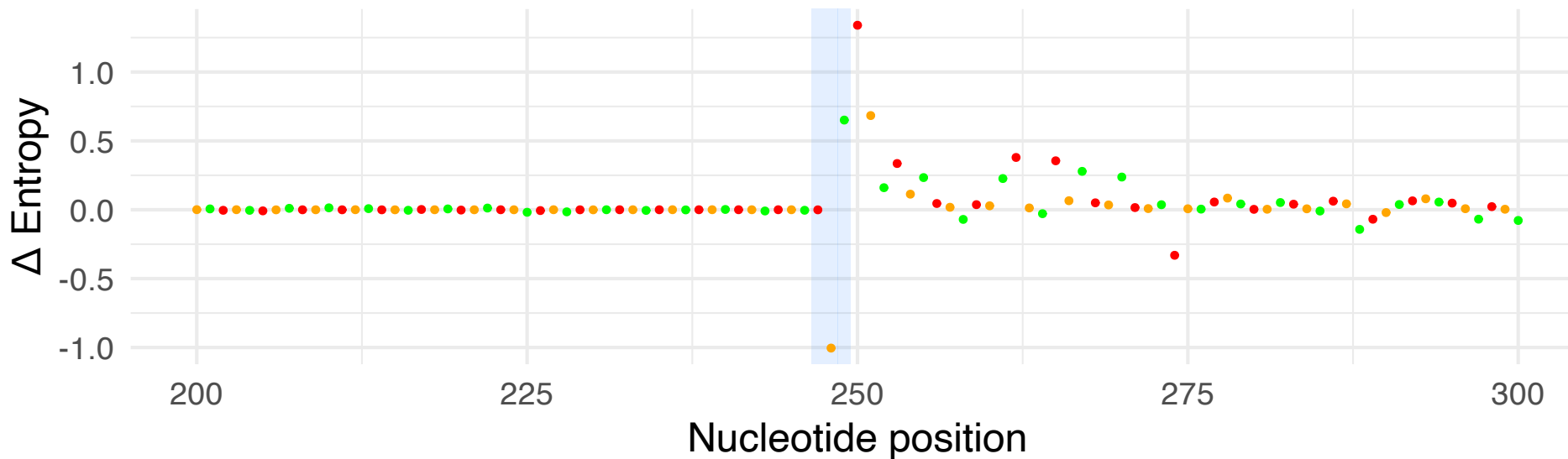
Entropy difference: 83_Stop vs 83_S1
