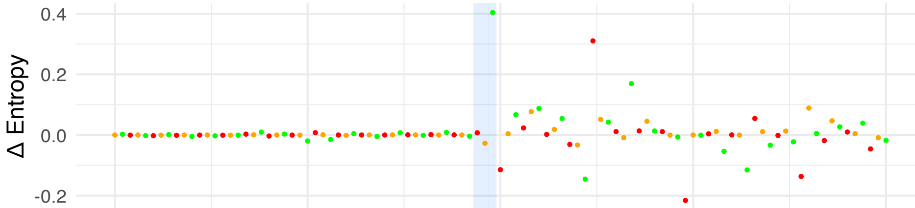
Entropy difference: 83_S2 vs 83_S1
