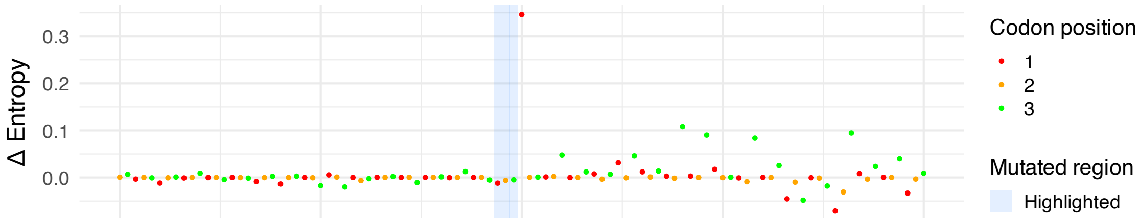
Entropy difference: 83_Stop vs 83_S1
