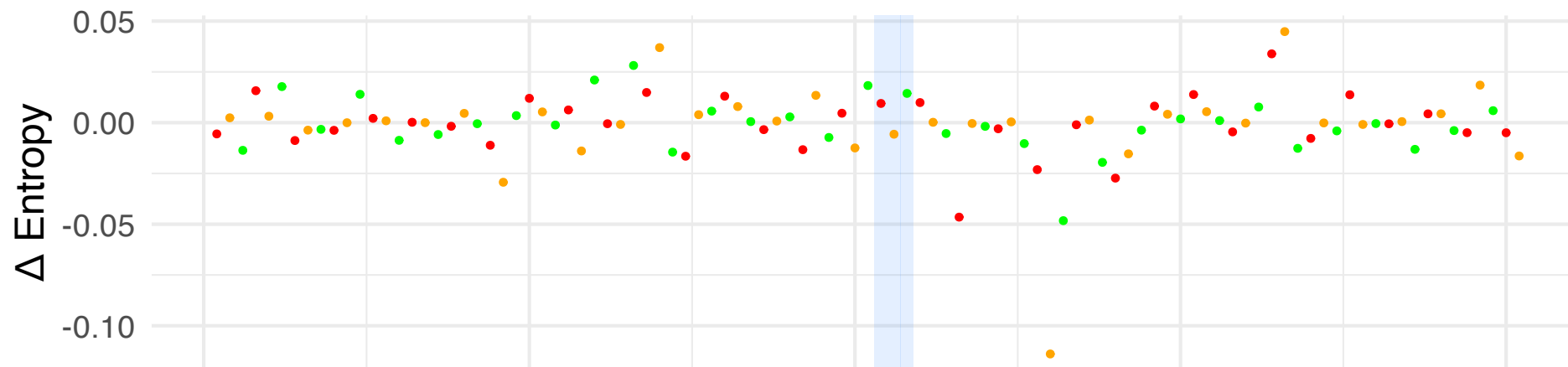
Entropy difference: 83_S1_shifted1r vs 83_S1
