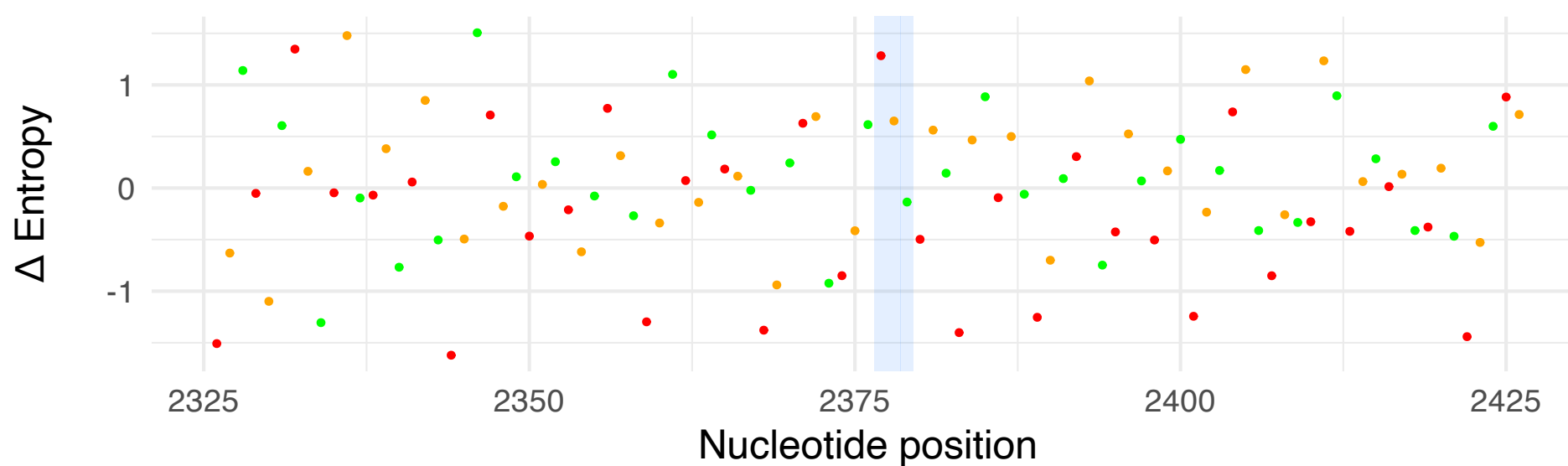
Entropy difference: 83_S1_shifted2r vs 83_S1
