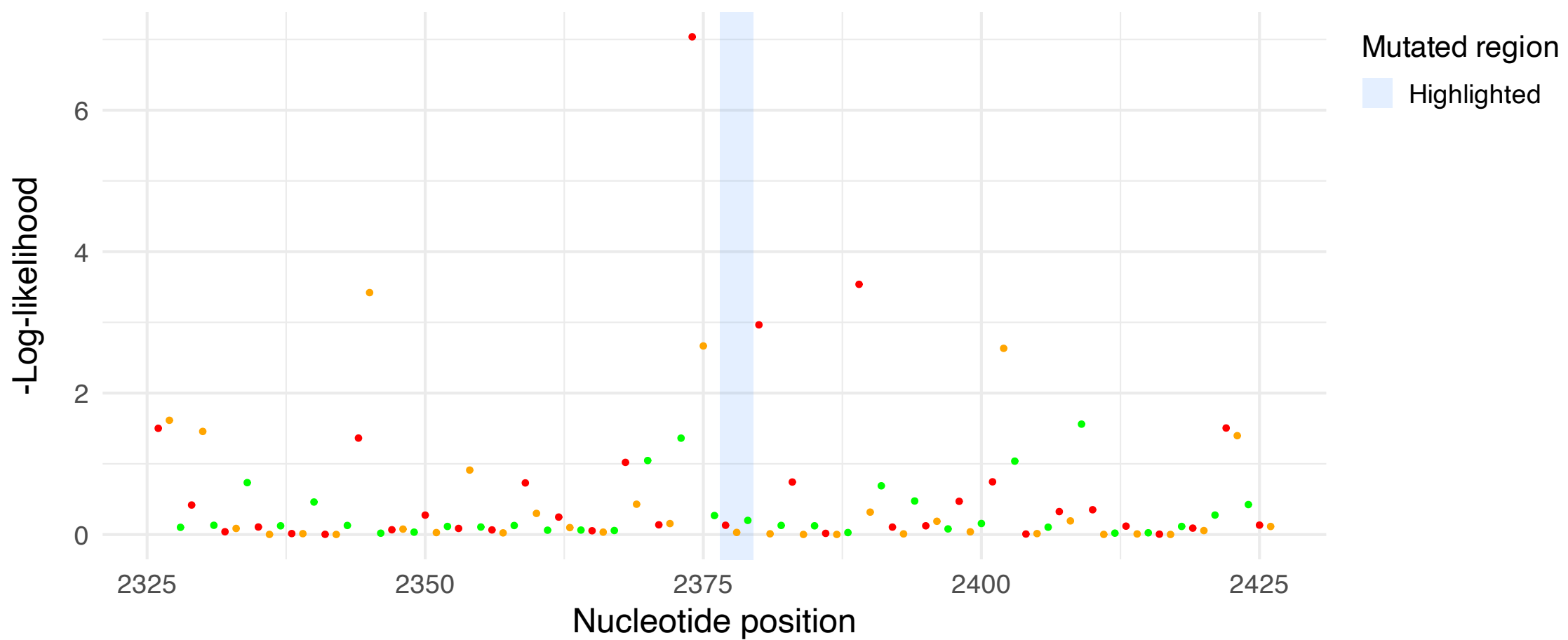
-Log-likelihood across positions 2326-2426 (83_S1)
