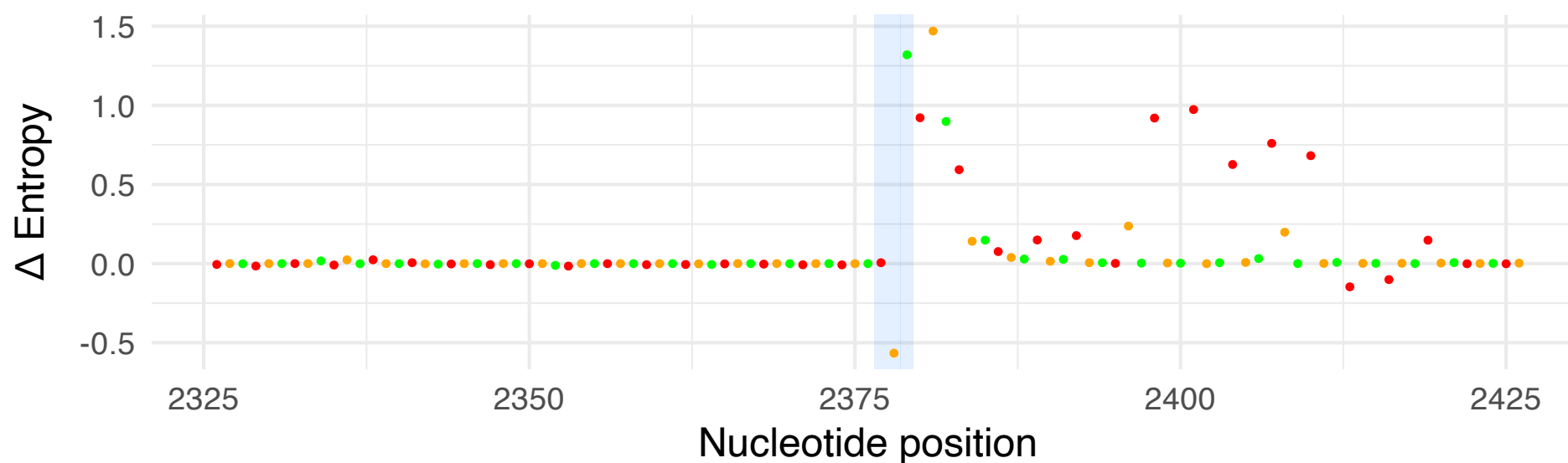
Entropy difference: 83_TGA_rc vs 83_AGC_rc
