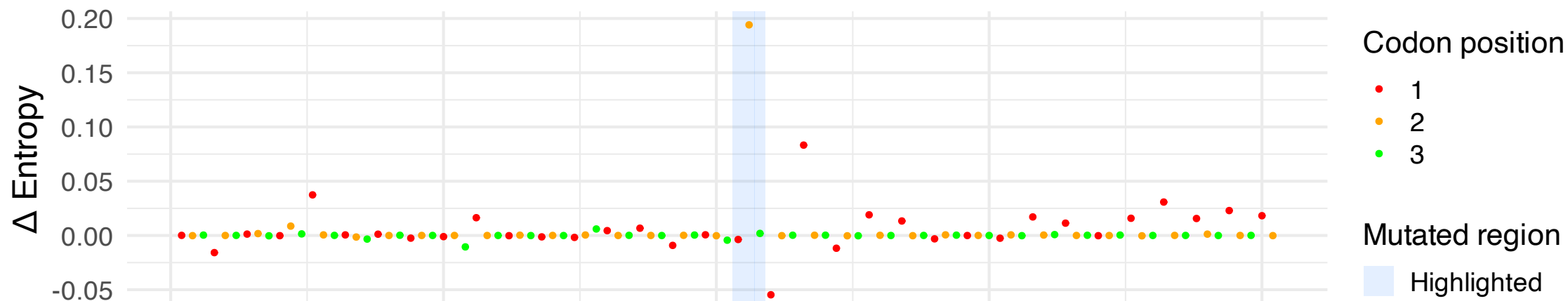
Entropy difference: 83_TGA_rc vs 83_AGC_rc
