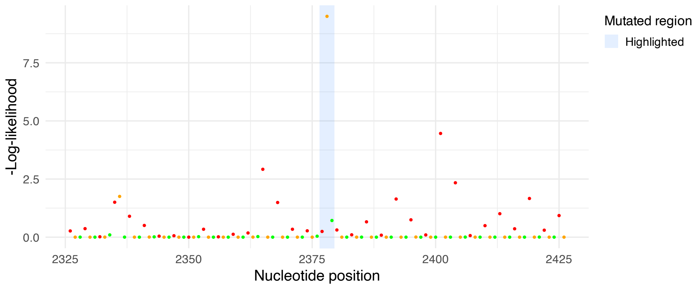
-Log-likelihood across positions 2326-2426 (83_ATC_rc)
