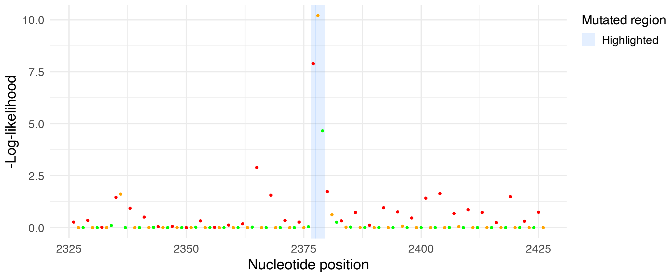
-Log-likelihood across positions 2326-2426 (83_TGA_rc)
