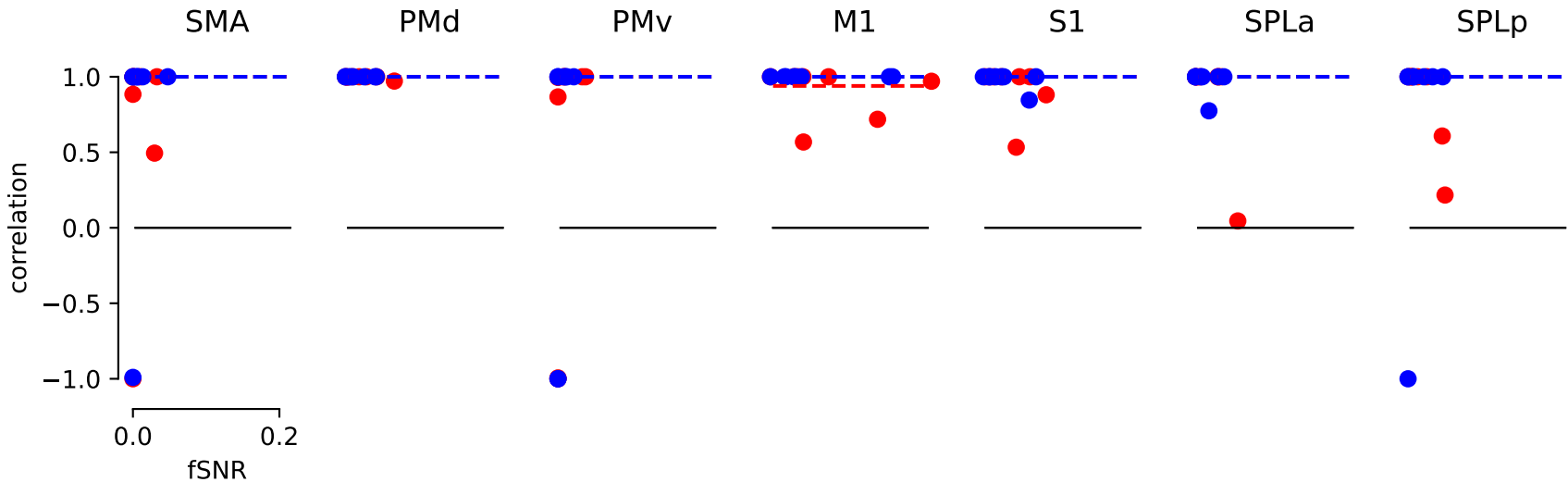
MLE correlation between sess 9 vs. 23
