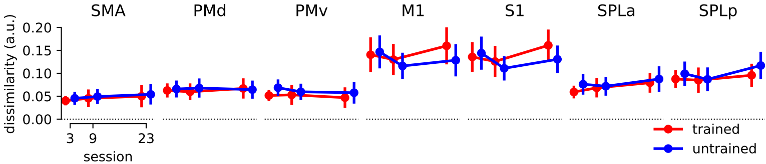
Average crossnobis dissimilarity between trained and untrained chords
