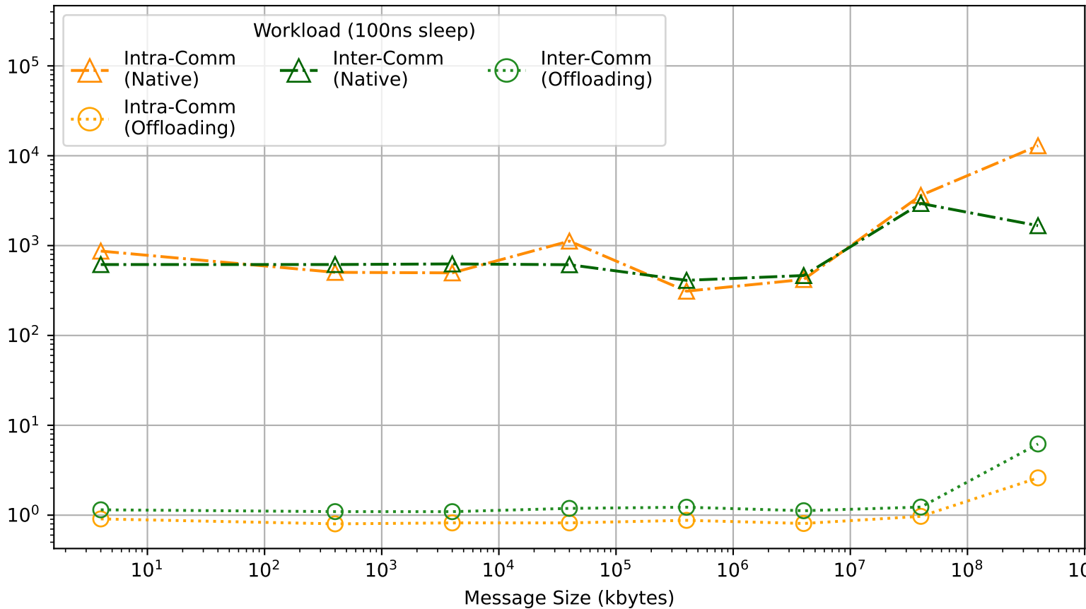
Overhead on HAWK: Intra- and Inter-Node Comm.
