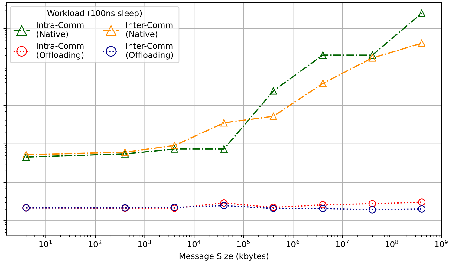
Overhead on SNG: Intra- and Inter-Node Comm.
