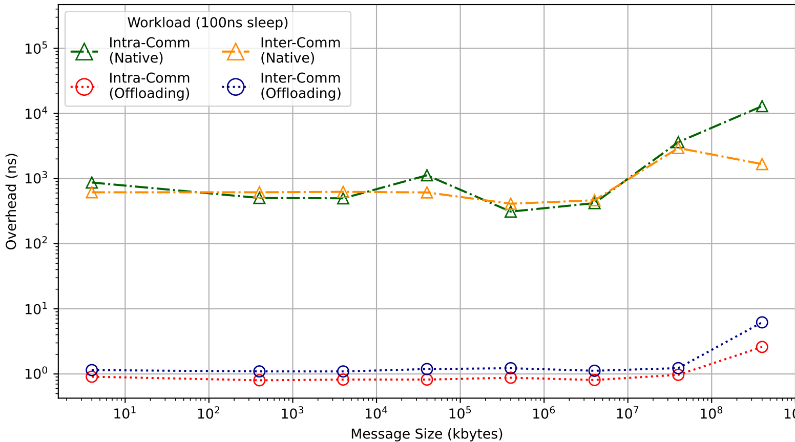
Overhead on HAWK: Intra- and Inter-Node Comm.
