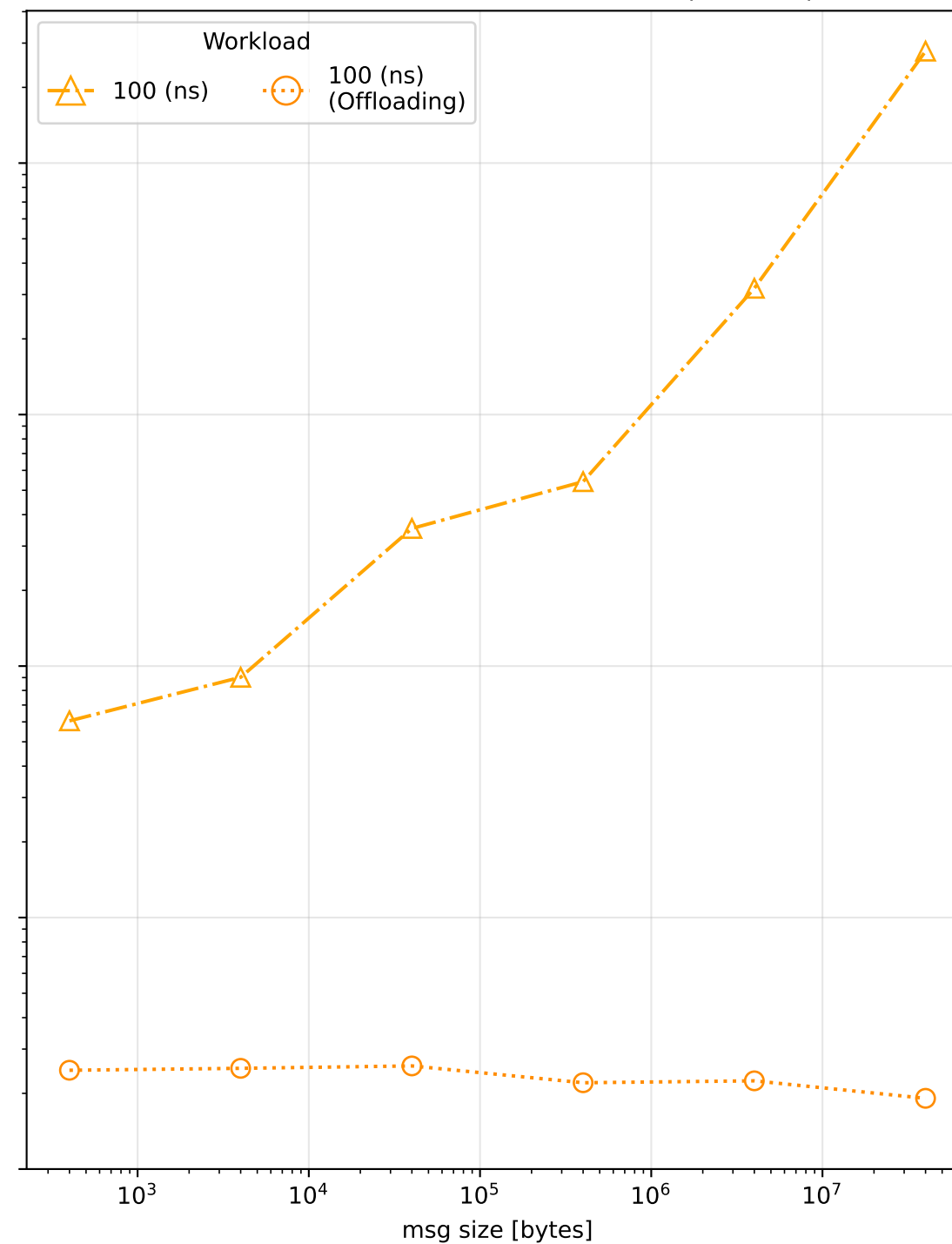
Intel-MPI Inter-Node Comm. on SNG (2 nodes)
