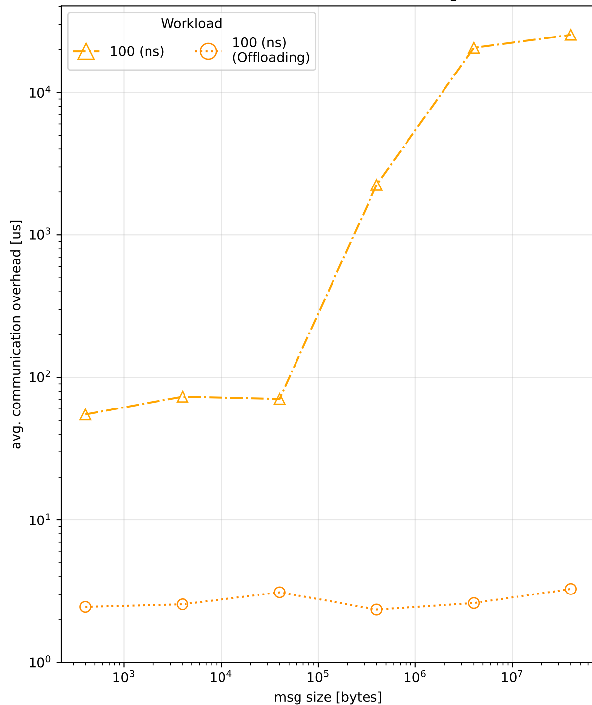
Intel-MPI Intra-Node Comm. on SNG (single node)
