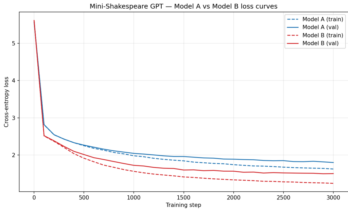
Loss curves
