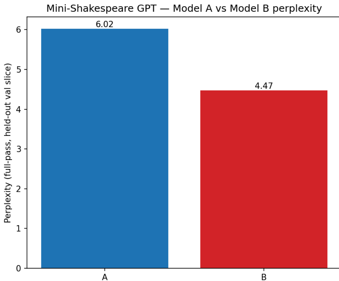
Perplexity comparison
