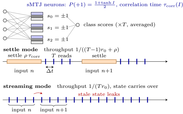
FIGURE 1. SBNN with sMTJ neurons (top) and the two operating modes (bottom). Settle mode pays \rho \tau_{corr} of relaxation per input; in streaming mode devices are never idle and the previous input's activation pattern persists in the device states.
