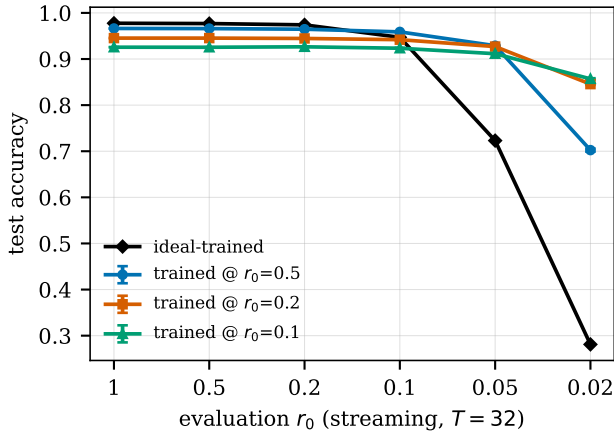
FIGURE 5. Correlation-aware training flattens the streaming failure curve (steady-state, T=32 ; mean \pm std over training and thermal seeds).
