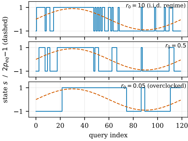
FIGURE 2. Telegraph SMTJ neuron at three sampling ratios, driven by a slowly varying firing probability (dashed). At r_0=10 samples are effectively i.i.d.; at r_0=0.05 the device returns long runs of stale state.
