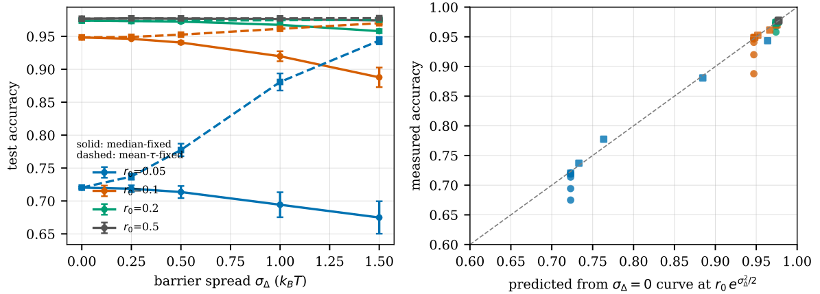
FIGURE 4. Left: apparent effect of dwell-time dispersion depends on the fixed population statistic: median-fixed (solid) degrades; mean- \tau_{\text{corr}} -fixed (dashed) appears to rescue ( T=32 , 5 chips, streaming). Right: the rescue is the centering's uniform rate offset in disguise: accuracy is predicted by the baseline ( \sigma = 0 ) curve evaluated at the median-device effective ratio r_0 e^{\sigma_\Delta^2/2} (mean- \tau_{\text{corr}} ) or r_0 (median), with dispersion contributing only a small residual penalty.
