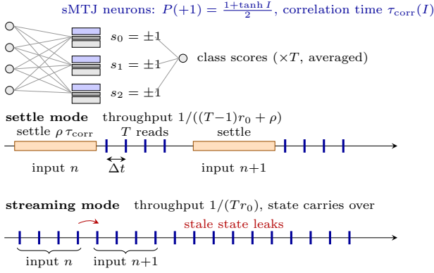
FIGURE 1. SBNB with sMTJ neurons (top) and the two operating modes (bottom). Settle mode pays \rho \tau_{\text{corr}} of relaxation per input; in streaming mode devices are never idle and the previous input's activation pattern persists in the device states.
