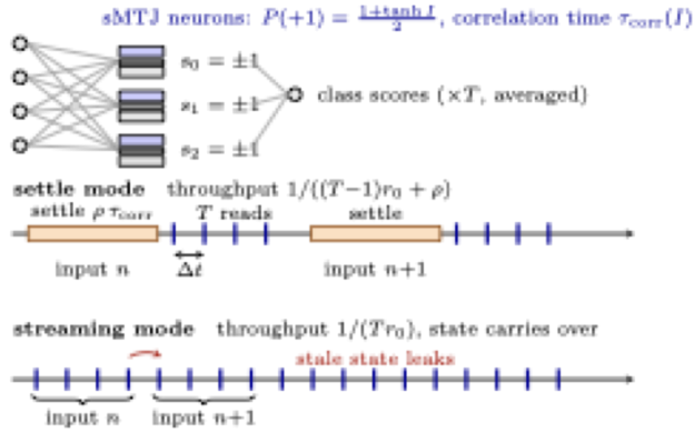
FIGURE 1. SBNN with sMTJ neurons (top) and the two operating modes (bottom). Settle mode pays \rho \tau_{\text{corr}} of relaxation per input; in streaming mode devices are never idle and the previous input's activation pattern persists in the device states.
