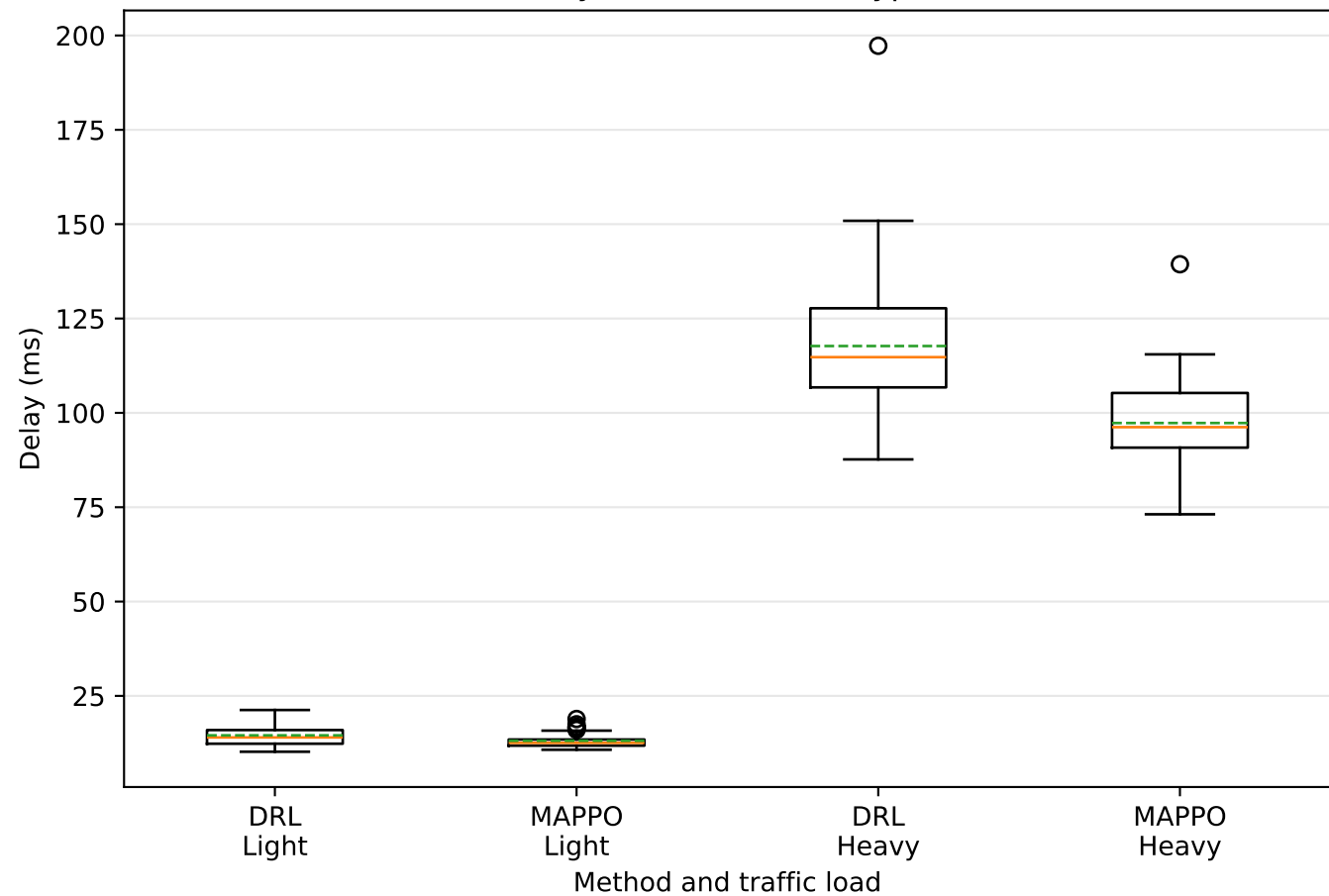
Delay (ms) — Service Type I
