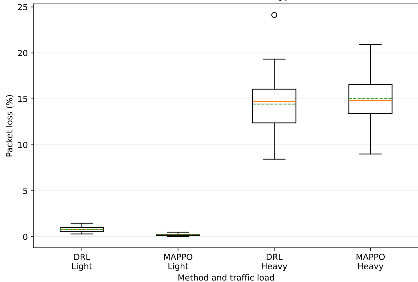
Packet loss (%) — Service Type IV
