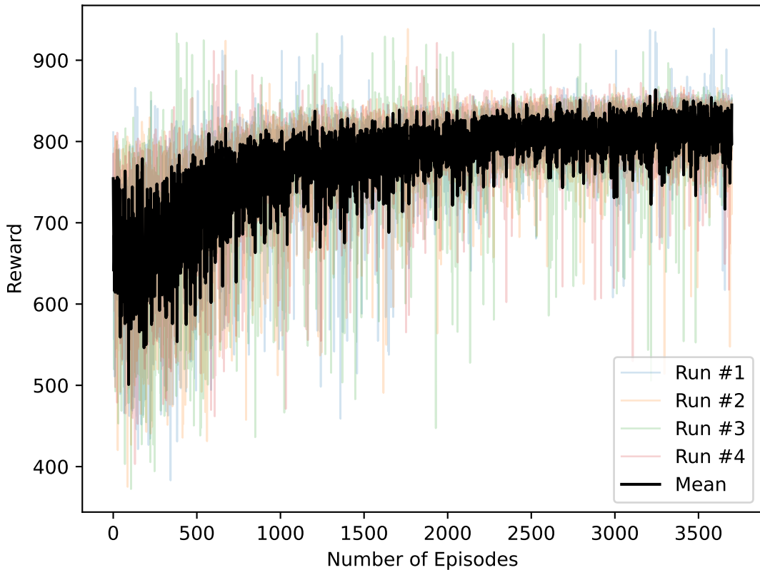
Adaptive PID Controller (Dynamic Model - Low Friction)
