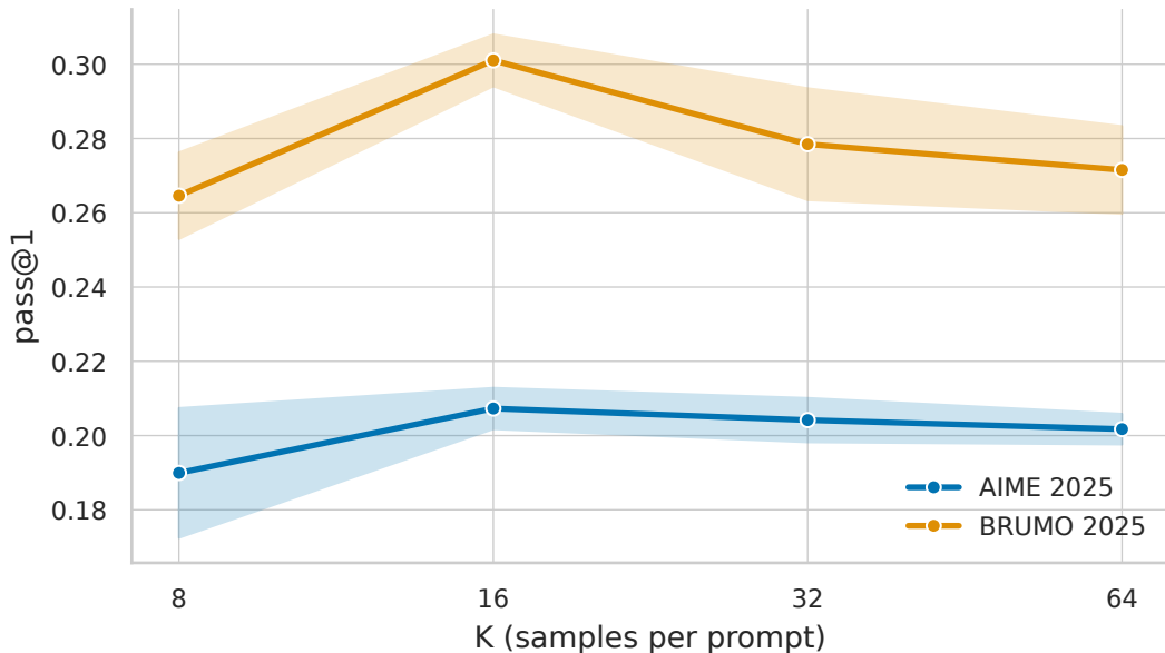
Baseline N/K sweep, best step per seed
