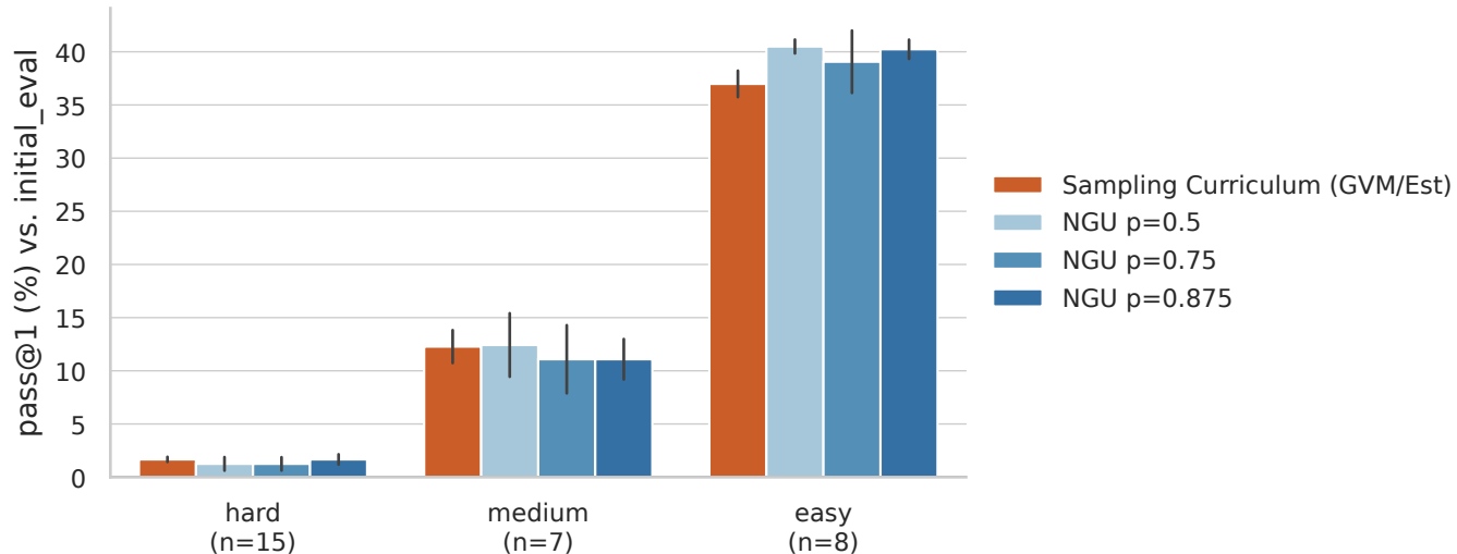
Sampling Curriculum (GVM/Est) vs. NGU p sweep, each run's best step (AIME)
