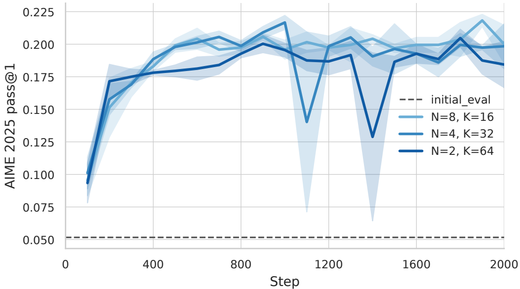
Baseline N/K sweep (grad norm 1.0)
