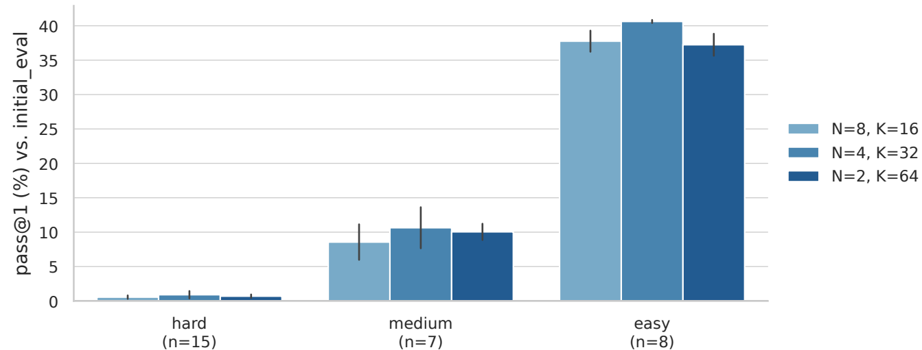
Baseline N/K sweep, each run's best step (AIME)
