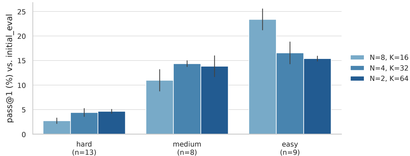
Baseline N/K sweep, each run's best step (BRUMO)
