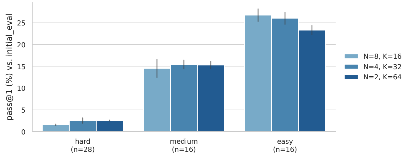
Baseline N/K sweep, each run's best step (AIME + BRUMO)
