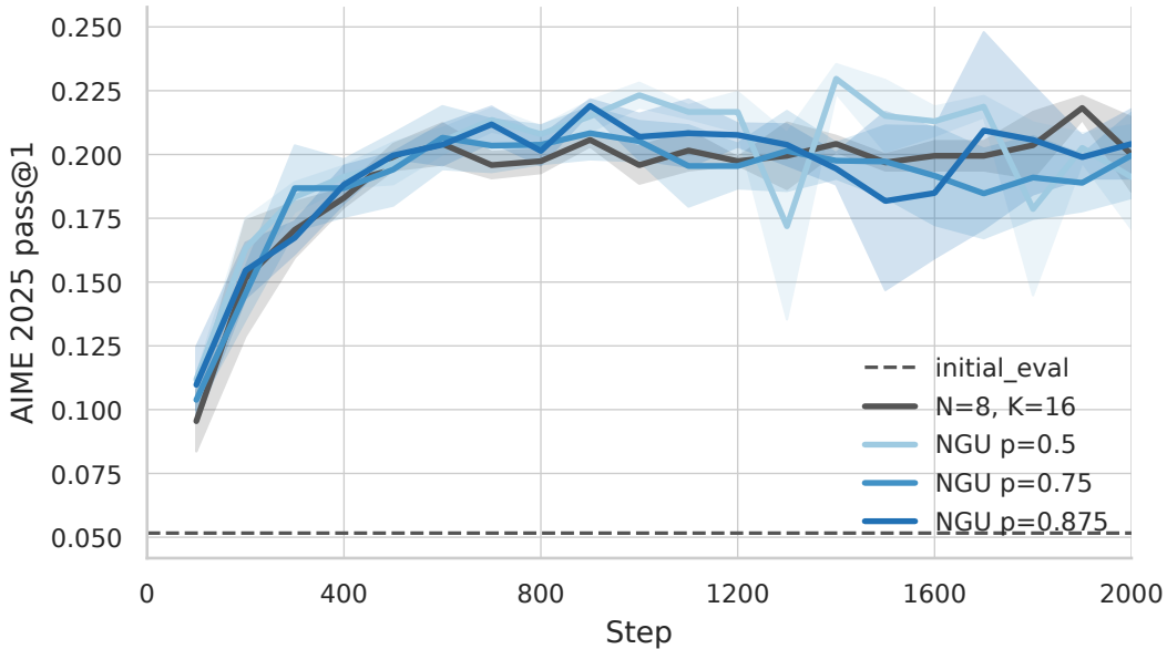
NGU p sweep (N=8, K=16, grad norm 1.0)
