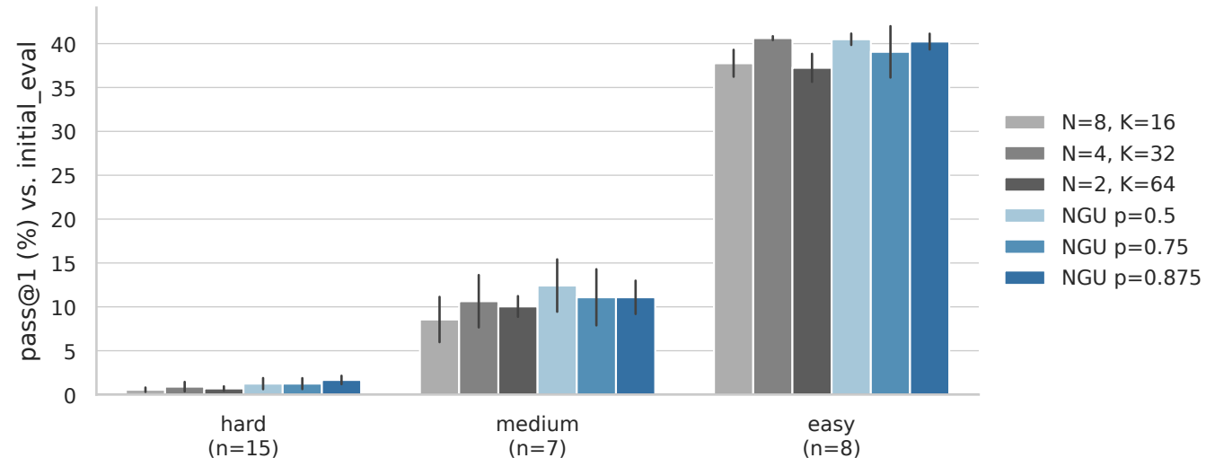
NGU p sweep vs. baselines, each run's best step (AIME)
