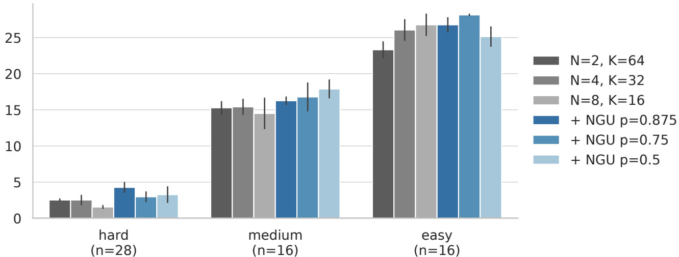
Pass@1 Improvement over Initial Model
