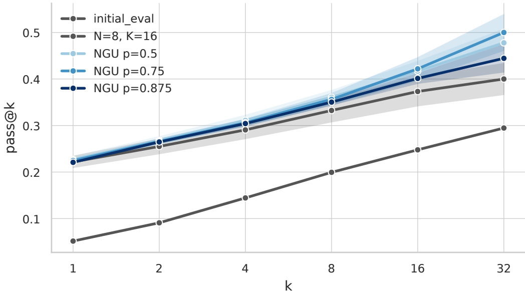
NGU p sweep, best step per seed
