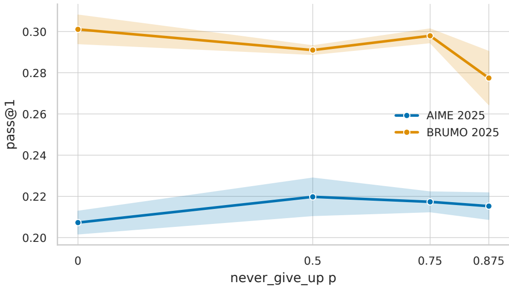
NGU p sweep (N=8, K=16), best step per seed
