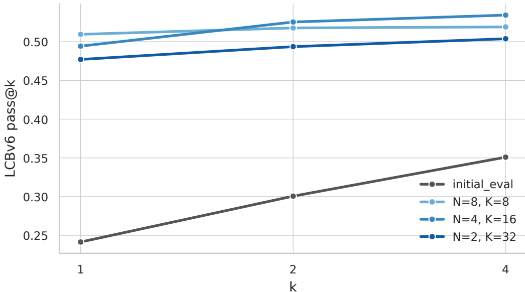
Baseline N/K sweep, each run's best step
