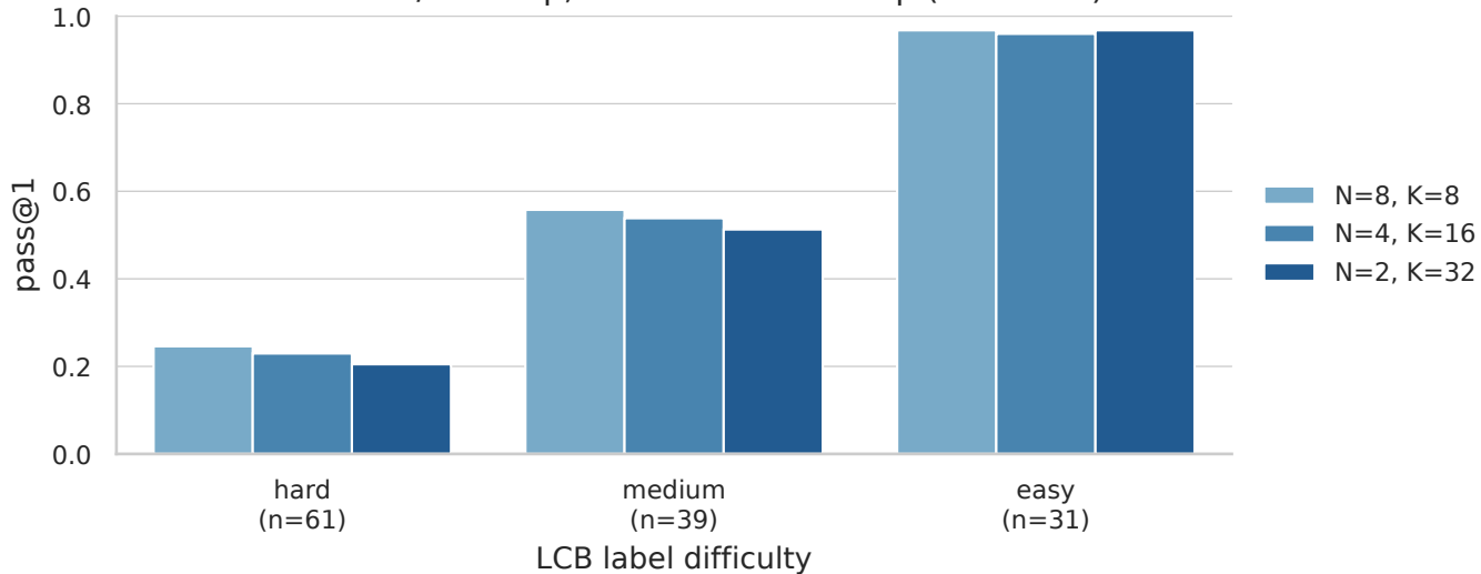
Baseline N/K sweep, each run's best step (LCB label)
