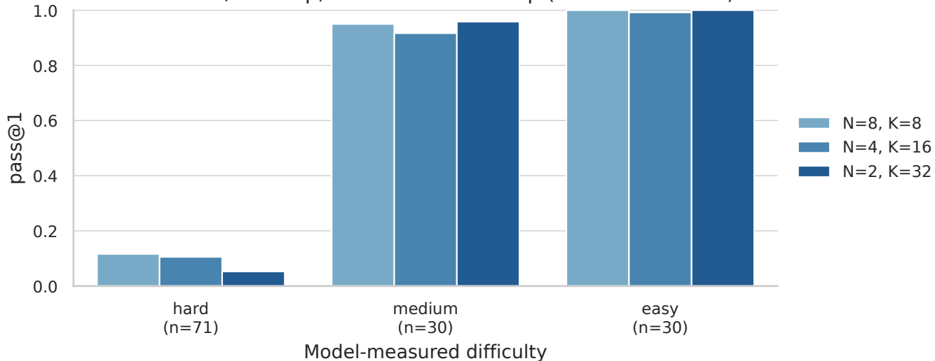
Baseline N/K sweep, each run's best step (Model-measured)
