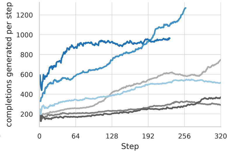
Batch composition over training (EMA smoothed)
