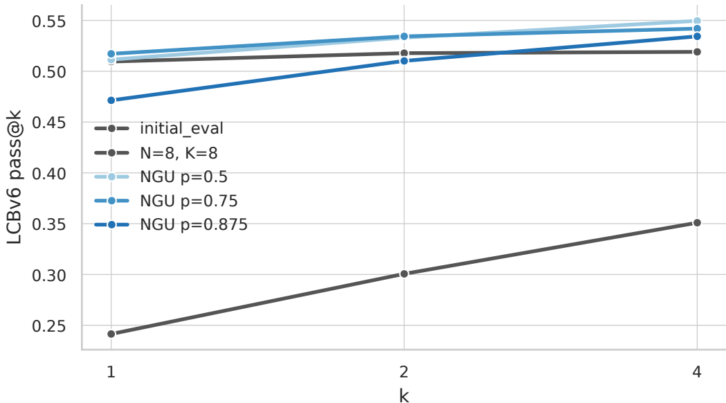
NGU p sweep, each run's best step
