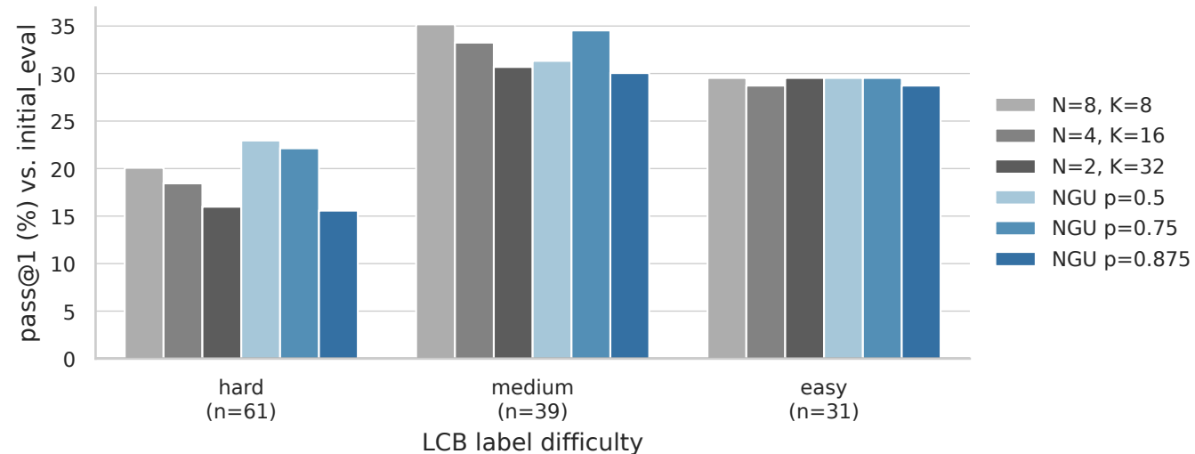
NGU p sweep vs. baselines, each run's best step (LCB label)
