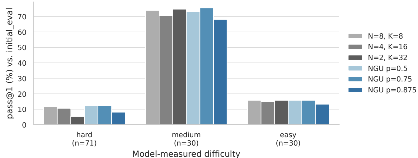
NGU p sweep vs. baselines, each run's best step (Model-measured)
