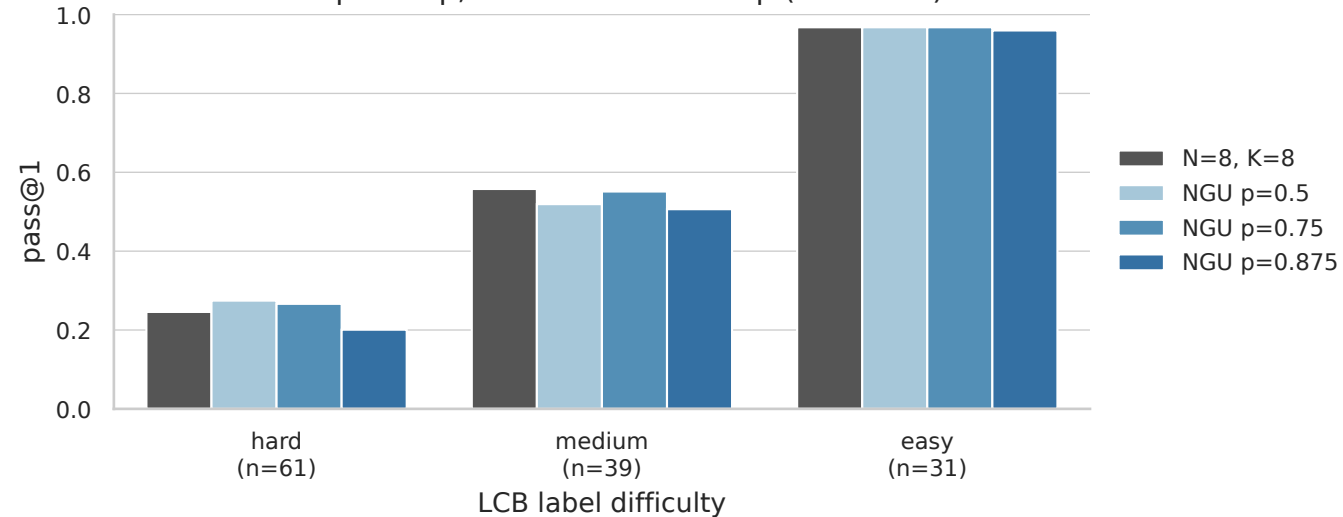
NGU p sweep, each run's best step (LCB label)
