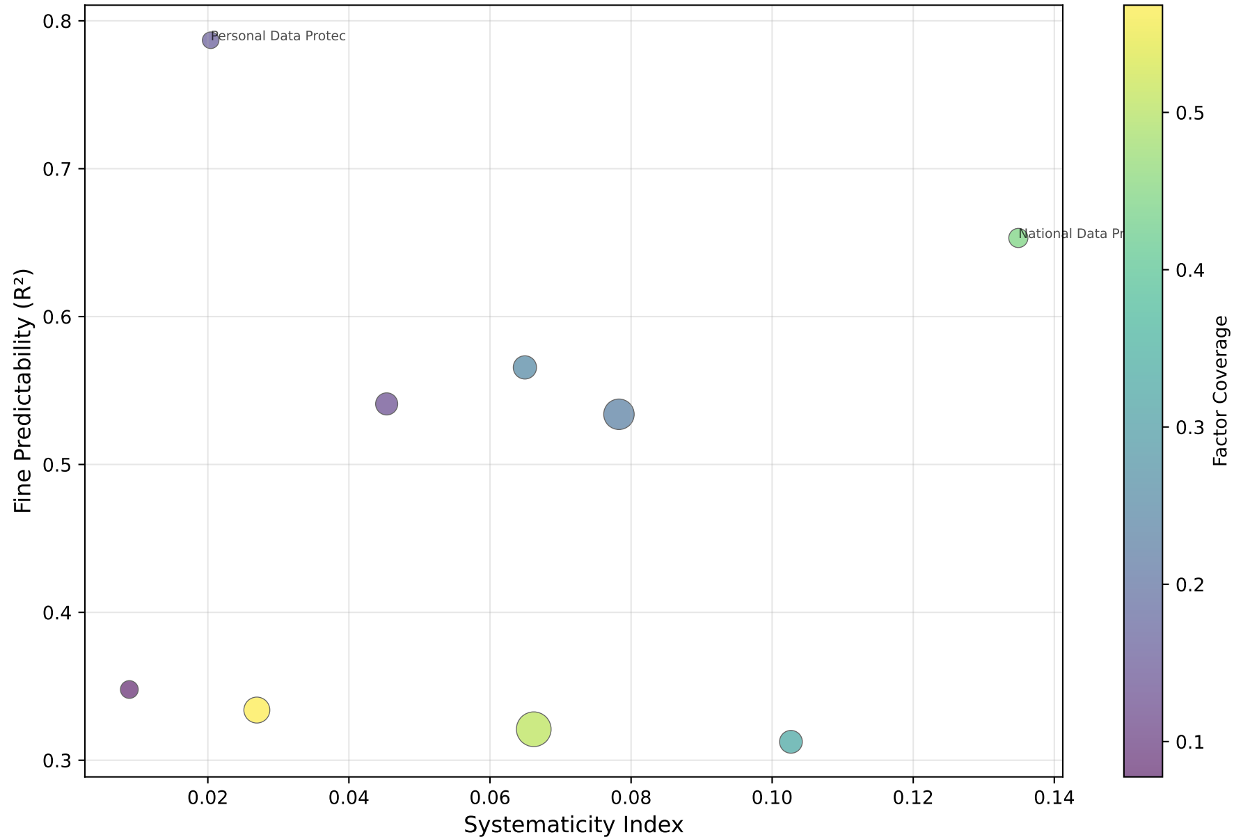
Authority Systematicity vs. Fine Predictability (bubble size = n decisions, color = coverage)
