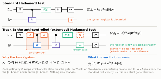
Figure 1: The anti-controlled Hadamard test. Conjugating the controlled- W by X on the ancilla makes W fire on the |0\rangle branch while the ordinary controlled- U fires on the |1\rangle branch, so the ancilla interferes two dynamics: \langle Z_a \rangle_\varphi = \text{Re}[e^{i\varphi}\chi_{AB}(t)] with \chi_{AB}(t) = \langle\psi|W^\dagger U|\psi\rangle . Setting W = I recovers the standard test. Construction after Ref. [1], Apps. B and E.
