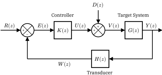
Figure 2. Closed-loop control system with controller, plant, disturbance input, and feedback transducer.
