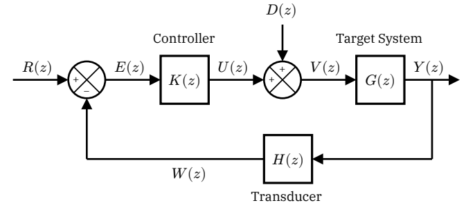
Figure 2. Closed-loop control system with controller, plant, disturbance input, and feed-back transducer.
