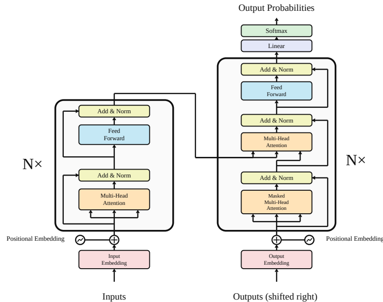
Figure 1. Transformer encoder-decoder block diagram (Vaswani et al., 2017).
