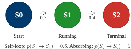
Figure 4. Three-state Markov chain; transition probabilities label the arcs.
