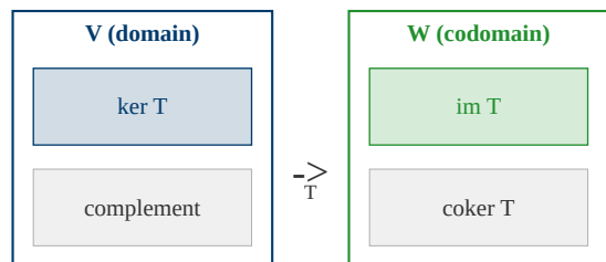
Figure 3. Kernel-image decomposition for a linear map T : V \rightarrow W .
