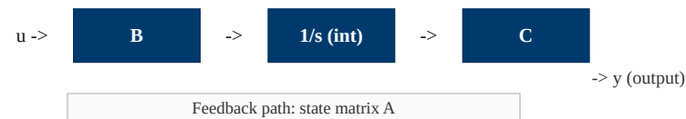
Figure 2. State-space block diagram: \dot{x} = Ax + Bu , y = Cx + Du .
