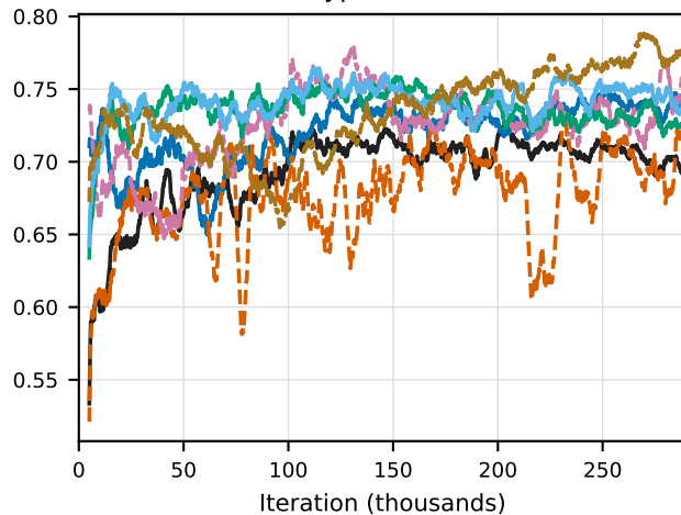
Prototype correlation
