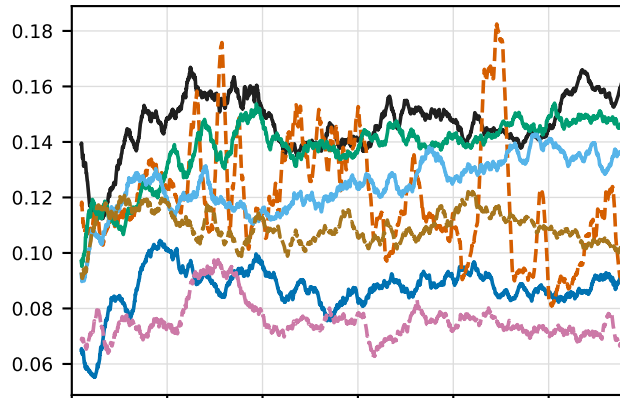
Prototype correlation
