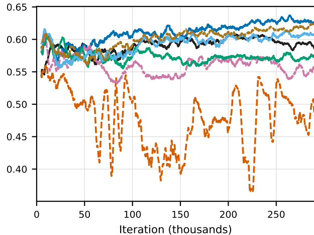
Real-fake loss
