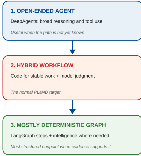
Figure 1. Intended PLaND evolution path. An initially open-ended workflow may become hybrid or mostly deterministic as stable behavior is validated. The figure is a design trajectory, not a claim that every workflow reaches the final stage.
